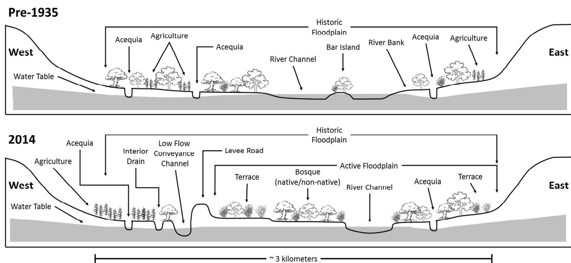
Figure 6. This figure shows a generalized cross section of the floodplain for both pre-1935 and 2014, looking north. There were major changes within the structure of the floodplain across the full study period.
